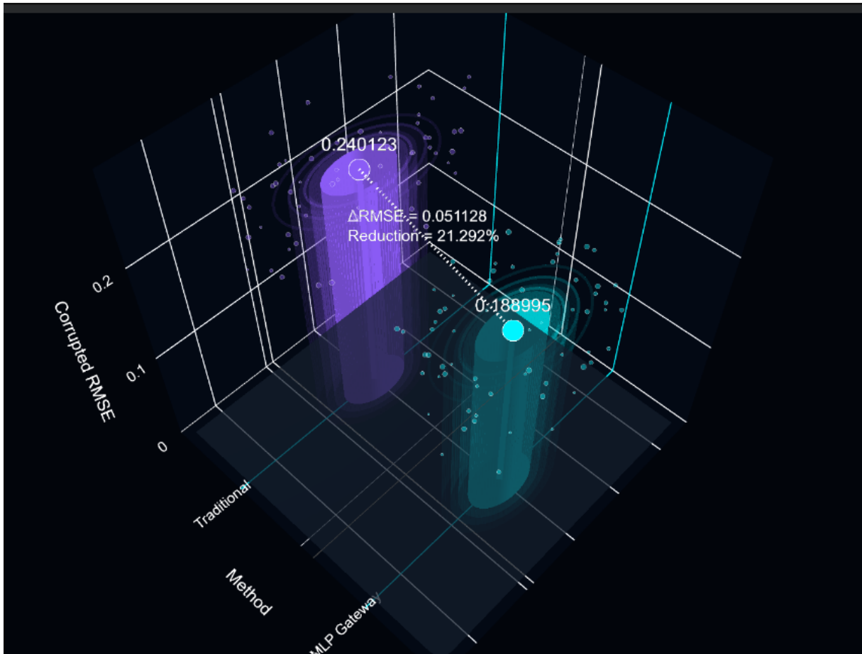
Figure 26: Historical complementary three-dimensional visualisation of the IPIP-NEO-300 corrupted-validation comparison. The figure is retained unchanged for research-history continuity and does not define the final P83.25 production performance.
